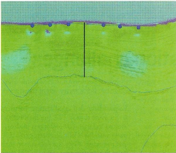
Figure 2. A preliminary inversion shows shallow resistive shale and deep resistive salt. Note the area to the west of the discovery well where the shallow resistor appears to be thicker.
