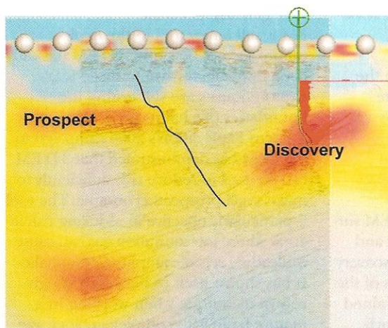
Figure 1. A depth section along a 2-D line shows agreement with borehole resistivity log from the discovery well and confirmation of prospect. (Images courtesy of EMGS Americas)
