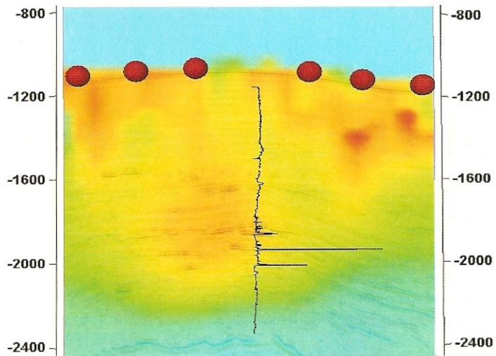
Figure 3. The final inversion around the discovery well shows greater detail. Note the resistive anomaly that coincides with the package of three seismic amplitudes and the three resistive layers observed on the well log.
